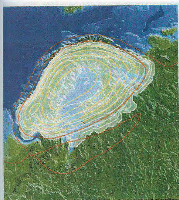
4a. 35 ka. OIS-3. (cold phase between Hengelo and Denekamp interstadials)
