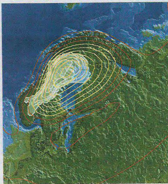
4c. 57 ka. OIS-3. Moerhoofd interstadial (Minimum ice limits)
