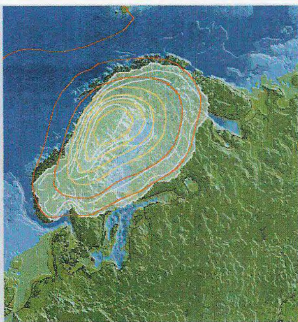
3b. 110 ka. OIS-5d. (cold stage)
